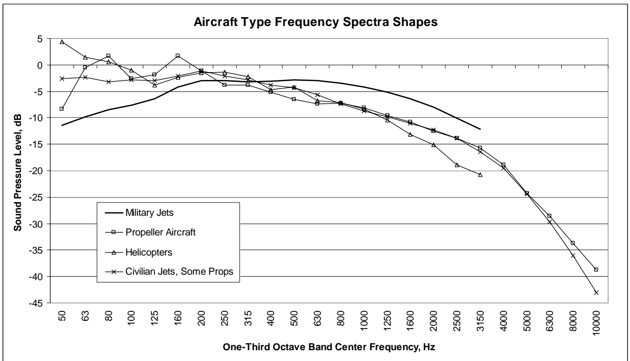
Figure 3-1. Spectra Summary
