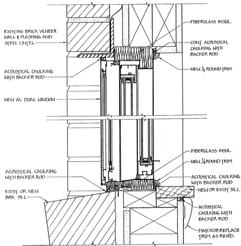
Figure C-1. Typical Combination Window Detail
