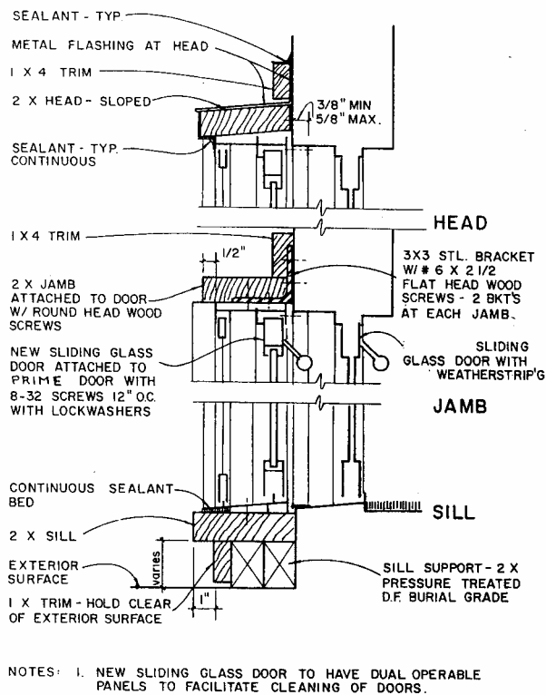
Figure C-3. Secondary Sliding Glass Door Detail
